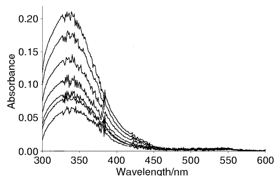
Fig. 2 Absorbance-time plots for the nitrosation of BSA ( 8.8 \times 10^{-5} mol dm -3 free thiol) with excess nitrous acid ( 1.83 \times 10^{-4} mol dm -3 ) in HCl (0.4 mol dm -3 ).
