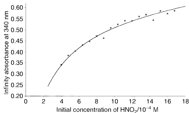
Fig. 4 Variation of A_\infty at 340 nm with initial [HNO 2 ] in the reaction of BSA with excess HNO 2 in HCl (0.4 mol dm -3 ).
