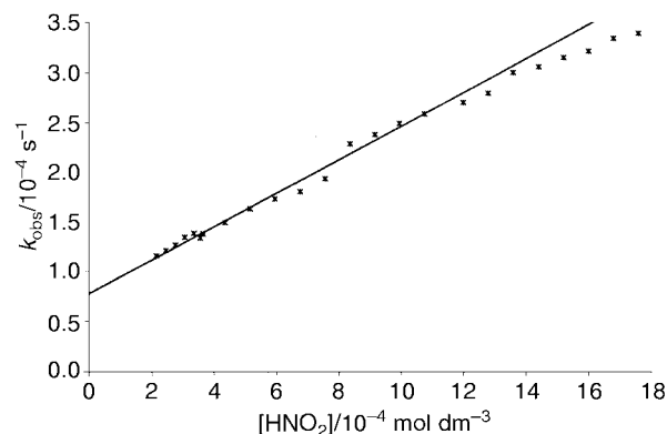
Fig. 5 Plots of k_{\text{obs}} against [HNO 2 ] in the reaction of BSA ( 7.7 \times 10^{-5} mol dm -3 free thiol) with HNO 2 in HCl (0.4 mol dm -3 ).
