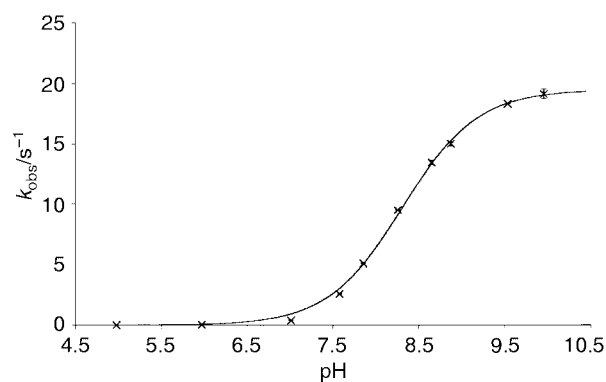
Fig. 1 Values of k_{\text{obs}} as a function of pH in the reaction of BSA with dipyridin-4-yl disulfide.
